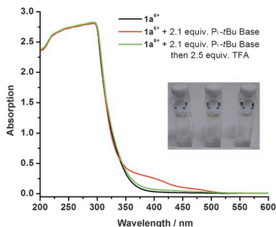
Figure 2. Change in UV/Vis absorption spectra of compound 1a (PF 6 ) 6 in CD 3 CN (0.39 mm) before deprotonation (black), after deprotonation with 2.1 equiv of P 1 -tBu base [17] (red) and after reprotonation with 2.5 equivalents of trifluoroacetic acid (TFA, green). Inset, from left to right side, shows the color change during this process.
